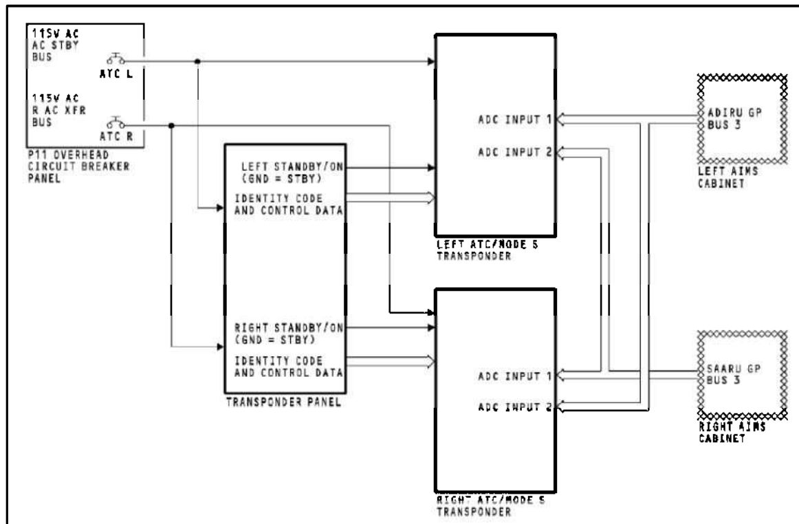
Figure 1.9B - ATC/Mode S Transponder Power System
